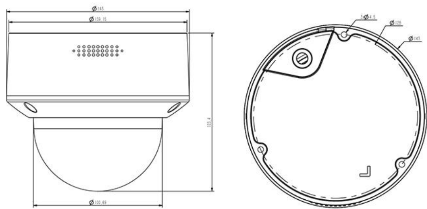
AD2Y01 Outline Dimensions
